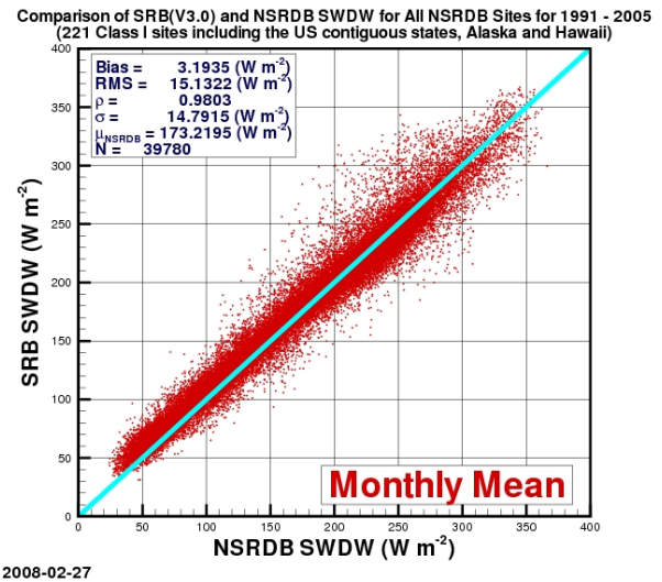
Figure 3. Scatter plot of SRB(V3.0)-NSRDB monthly mean surface downward shortwave flux comparison.
