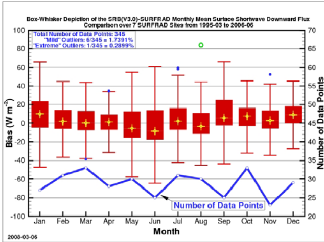
Figure 10. A box-whisker presentation similar to Figure 8 but this time comparing monthly averaged SRB(V3.0) to SurfRad measurements.
