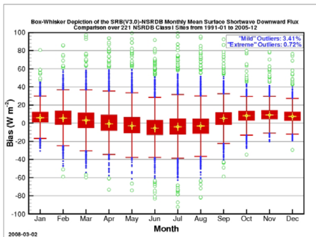
Figure 8. A box-whisker presentation of the SRB(V3.0)-NSRDB monthly mean surface downward shortwave flux comparison bias for January through December.
