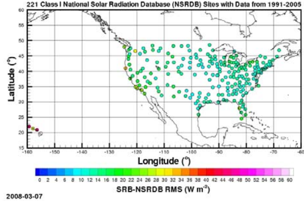
Figure 2. SRB(V3.0)-NSRDB monthly mean surface downward shortwave flux comparison RMS on a site-by-site basis.
