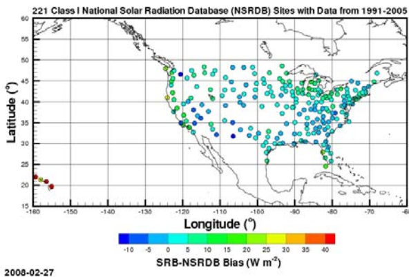
Figure 1. SRB(V3.0)-NSRDB monthly mean surface downward shortwave flux comparison bias on a site-by-site basis.
