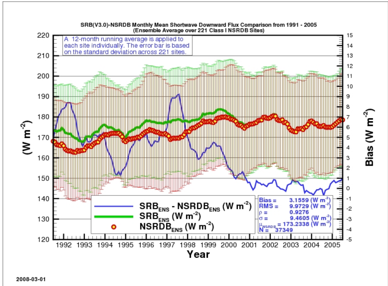
Figure 11. A 12-month running average is applied to each site individually and then an ensemble average across the 221 sites is performed on both SRB(V3.0) and NSRDB data. The error bars are based on standard deviation of each set respectively. Note that the first five (5) months in 1991 and last six (6) months of 2005 disappear from the picture after the 12-month running average. Also, note that METSTAT model estimates comprise the nearly all the NSRDB values from 1991-1997 and SUNY model estimates from 1998-2005.
