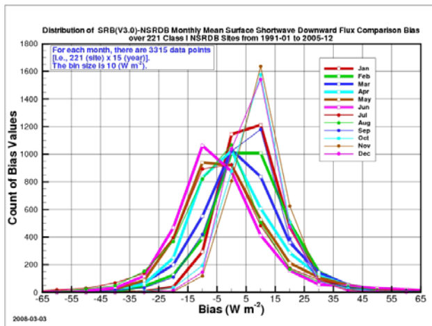
Figure 7. Distribution of bias January through December. Each month has 3,315 data points, i.e., 221 sites time 15 years.
