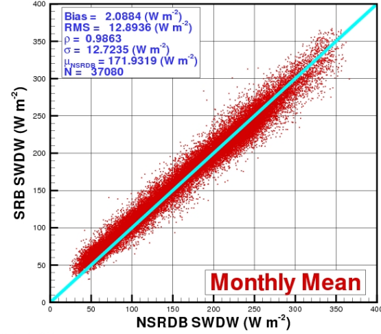
Comparison of SRB(V3.0) and NSRDB SWDW for All NSRDB Sites for 1991 - 2005 (221 Class I sites including the US contiguous states, Alaska and Hawaii)
