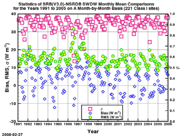
Figure 6. SRB(V3.0)-NSRDB monthly mean surface downward shortwave flux bias, RMS and correlation coefficient on a month-by-month basis.
