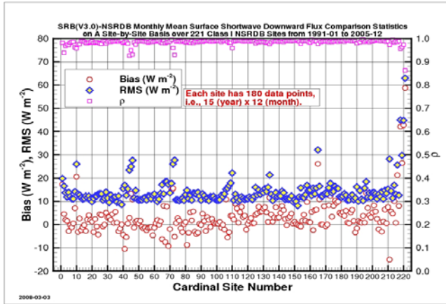
Figure 4. SRB(V3.0)-NSRDB monthly mean surface downward shortwave flux bias, RMS and correlation coefficient on a site-by-site basis.
