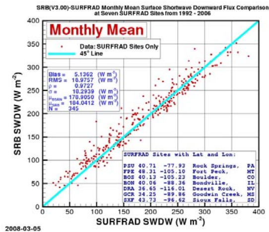
Figure 9. Scatter plot of the monthly averaged SurfRad solar irradiance measurement versus the NASA SRB estimate for the 1^\circ \times 1^\circ grid box containing the site. The sites are listed on the plot.
